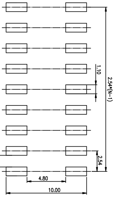
RECOMMENDED P.C.B. LAYOUT (TOP VIEW)
